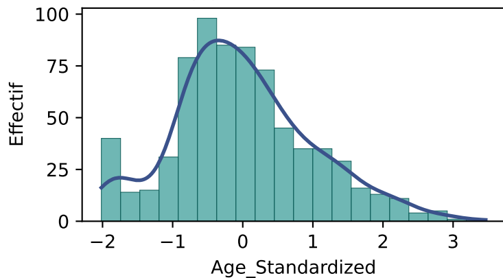
(b) Standardisation
